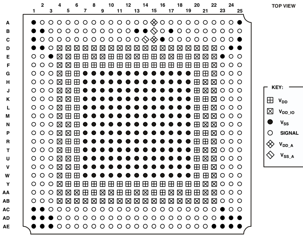
Figure 41. 625-Ball PBGA Pin Configurations (Top View, Summary)
